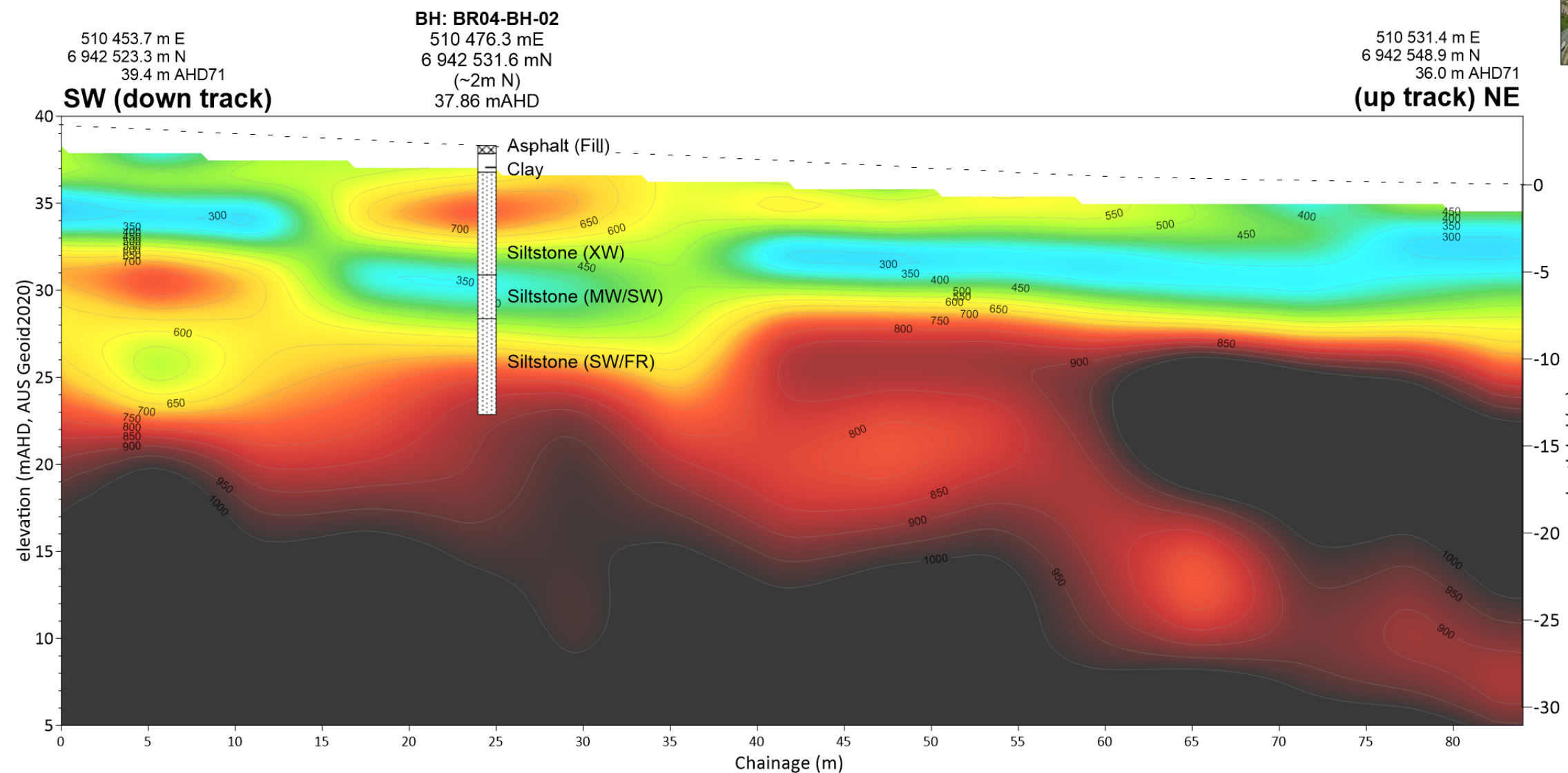
Seismic Line MASW AU-GP 134
